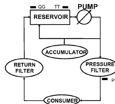
Figure 1 General Schematic of a Hydraulic System (Vianna, 2008).
