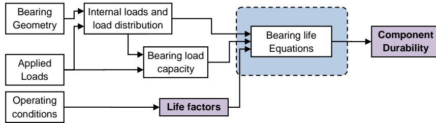
Figure 3. Approach to usage-based bearing lifing used by AVDPIP
