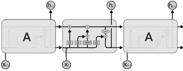
Figure 15. Repeating modules in LSTMs
