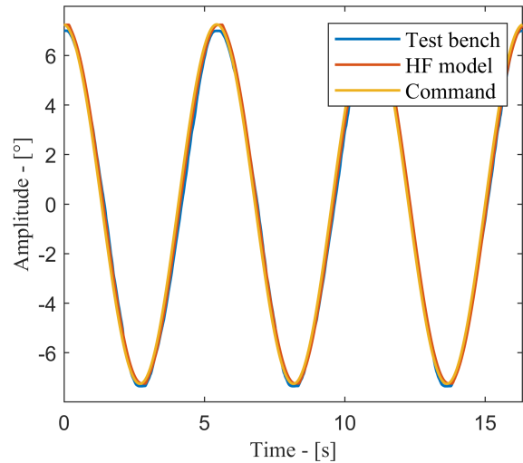
Figure 9. Commanded position, Simulink Model and Test Bench in zero backlash condition.
