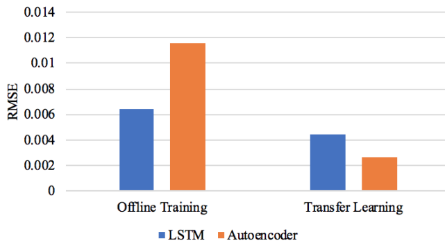
Figure 7. The RSME between the normalized actual and predicted values of all measured variables in two training modes – off-line training and transfer learning.
