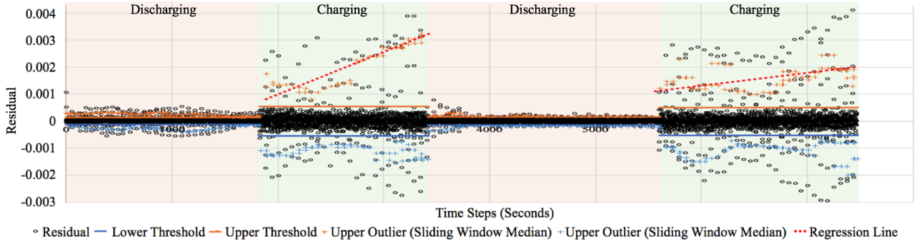
Figure 8. The residuals are decomposed from the reconstruction errors between auto-encoder inputs and outputs.
