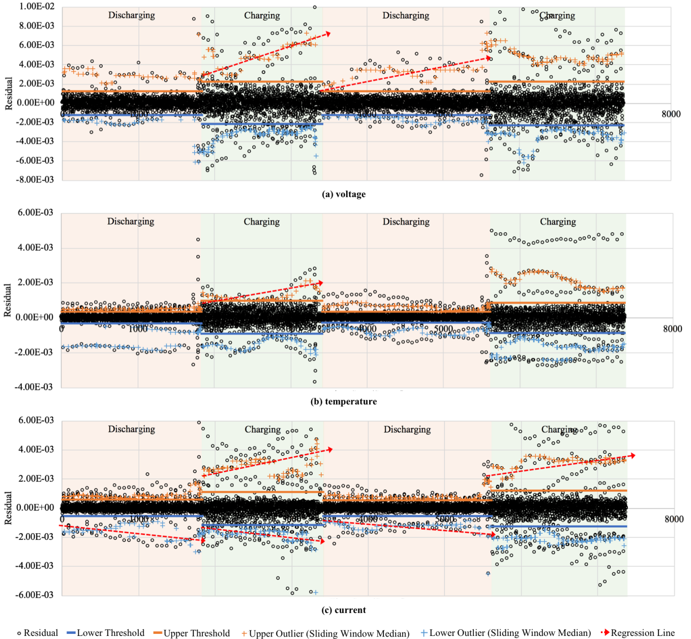
Figure 9. The residuals are decomposed from the time series of differences between actual and predicted voltage, temperature and current values (LSTM) outputs
