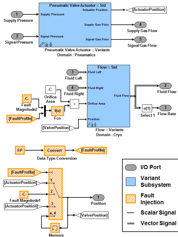
Figure 2. Control valve (CV) component model
