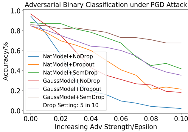
Figure 3. Failure Status Binary Accuracy under Increasing Adversarial Attack Strength
