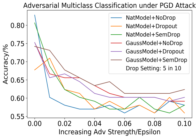
Figure 4. Health Status Multiclass Accuracy under Increasing Adversarial Attack Strength
