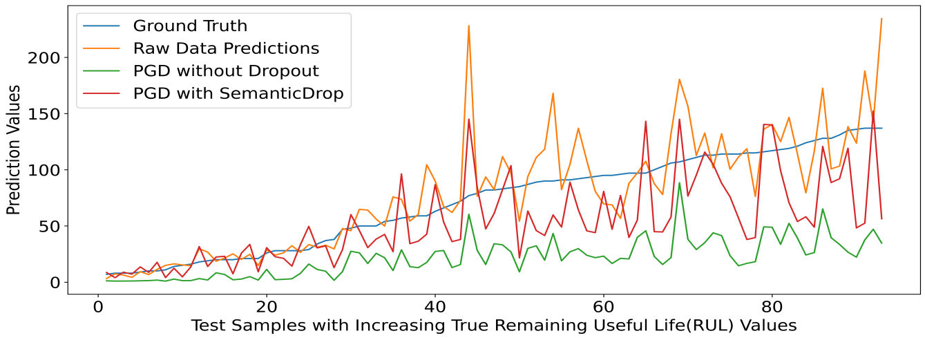
Figure 10. Regression Results (with GN) under Prediction Minimization PGD Adversarial Attack with advEps = 0.05(5\%)
