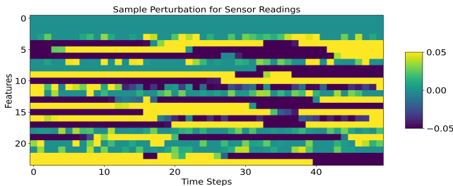
Figure 8. Example Adversarial Perturbation under Maximum Magnitude Constraint advEps = 0.05(5\%)
