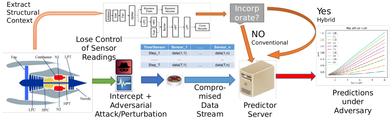
Figure 1. Overall Workflow for Robustness Evaluation of Deep Learning-based Prognostics on Conventional & Hybrid Models (with Randomization and Structural Contexts)
