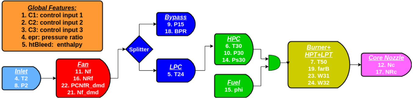
Figure 2. Groups of Features Along Layout Components (one color per group)
