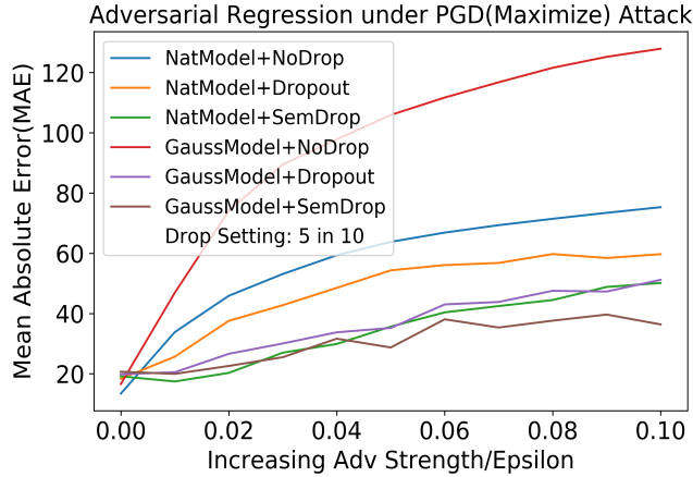
Figure 7. Remaining Useful Life Prediction Mean Absolute Error under Prediction Maximization Attack
