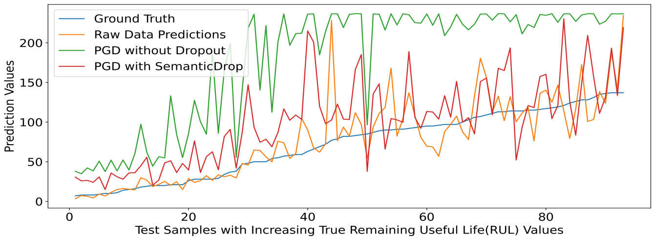
Figure 11. Regression Results (with GN) under Prediction Maximization PGD Adversarial Attack with advEps = 0.05(5\%)
