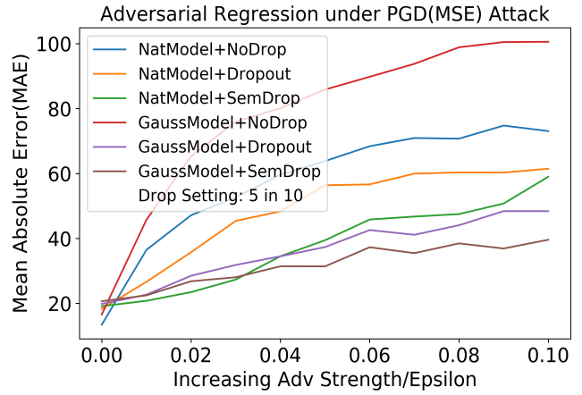
Figure 5. Remaining Useful Life Prediction Mean Absolute Error under Deviation Maximization Attack
