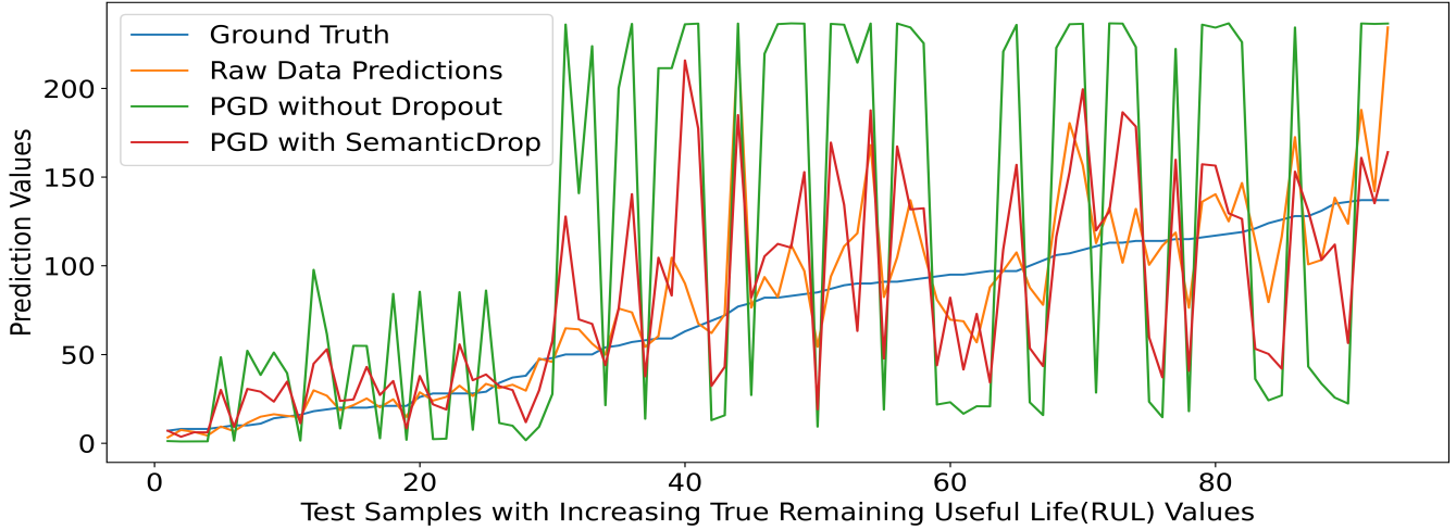
Figure 9. Regression Results (with GN) under Deviation Maximization PGD Adversarial Attack with advEps = 0.05(5\%)
