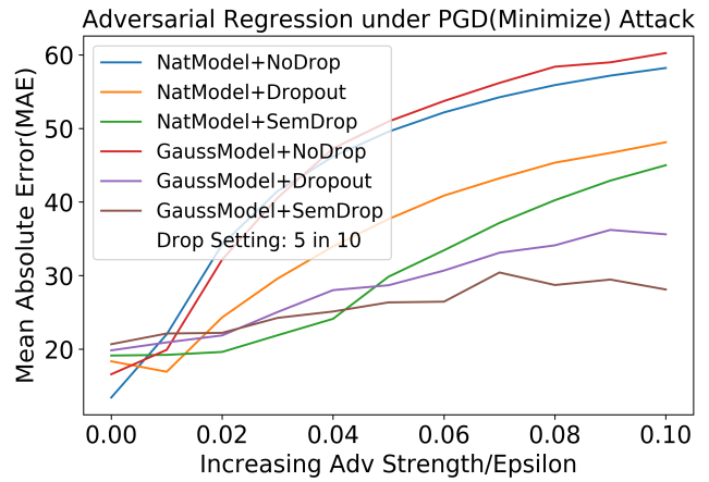
Figure 6. Remaining Useful Life Prediction Mean Absolute Error under Prediction Minimization Attack
